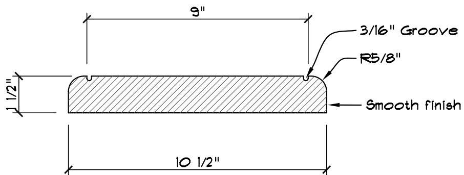
SECTION VIEW
