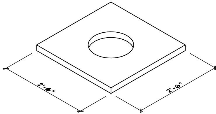
ISO VIEW
