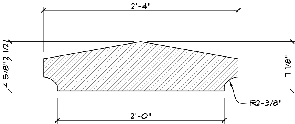
SECTION VIEW
