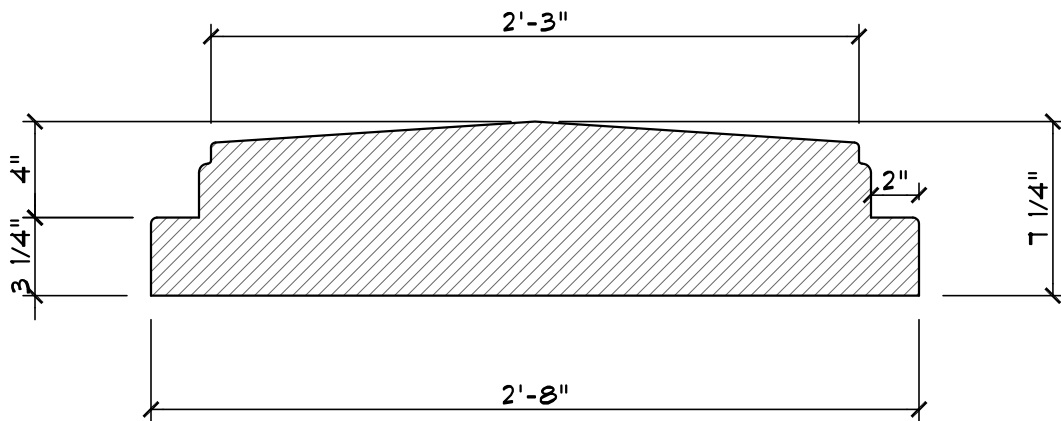
SECTION VIEW
