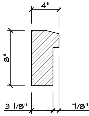
SECTION VIEW
