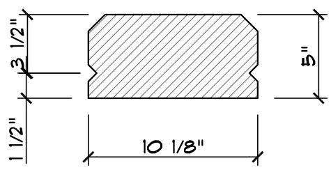
SECTION VIEW
