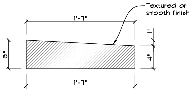
SECTION VIEW
