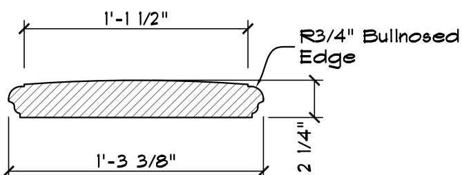
SECTION VIEW
