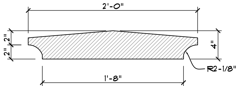
SECTION VIEW
