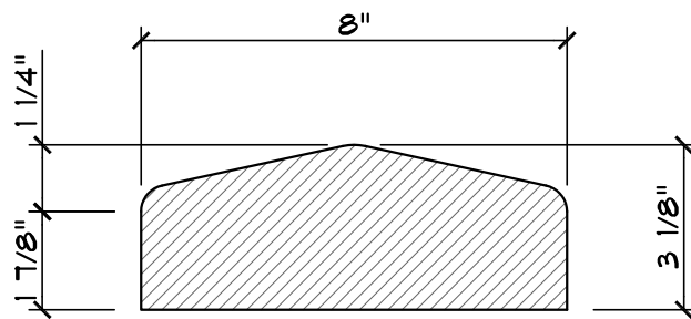
SECTION VIEW
