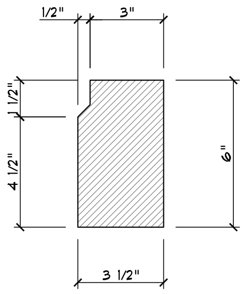
SECTION VIEW
