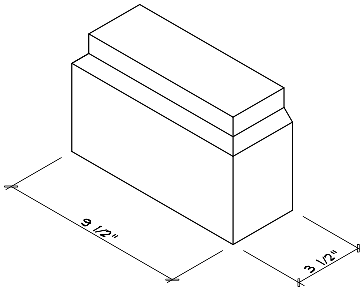
ISO VIEW
