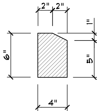
SECTION VIEW
