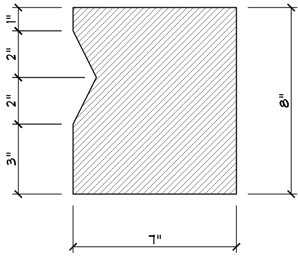
SECTION VIEW
