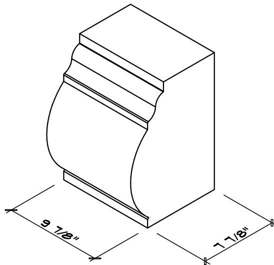
ISO VIEW
