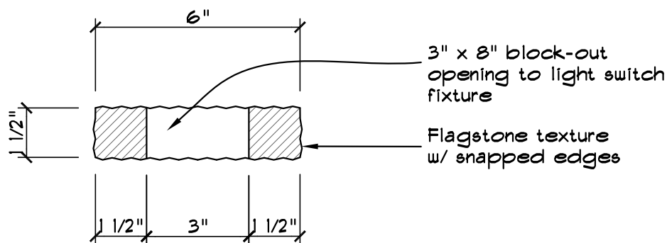
SECTION VIEW
