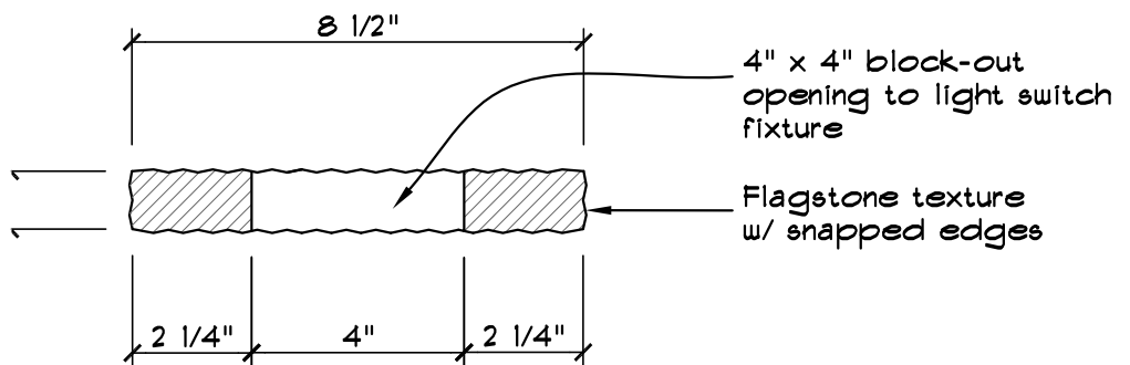
SECTION VIEW
