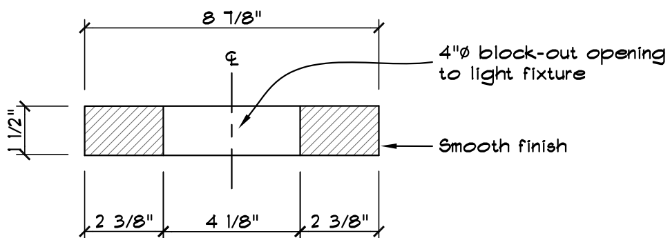
SECTION VIEW
